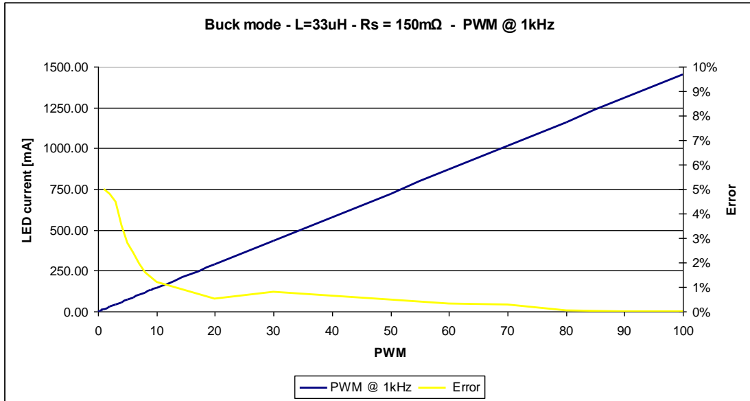
Figure 10. LED Current Linearity and Accuracy with PWM Dimming at 1kHz
