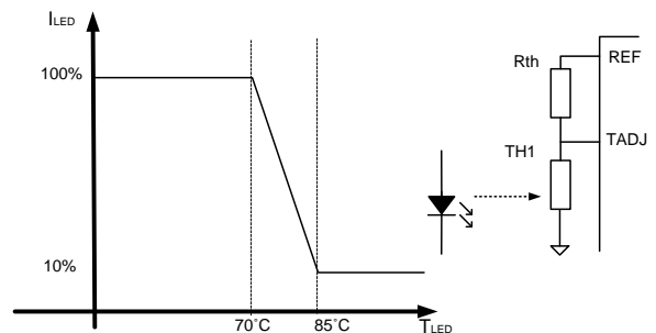
Thermal network response in Buck configuration with: R th = 1.8kΩ and TH1=10kΩ (beta =3900)
