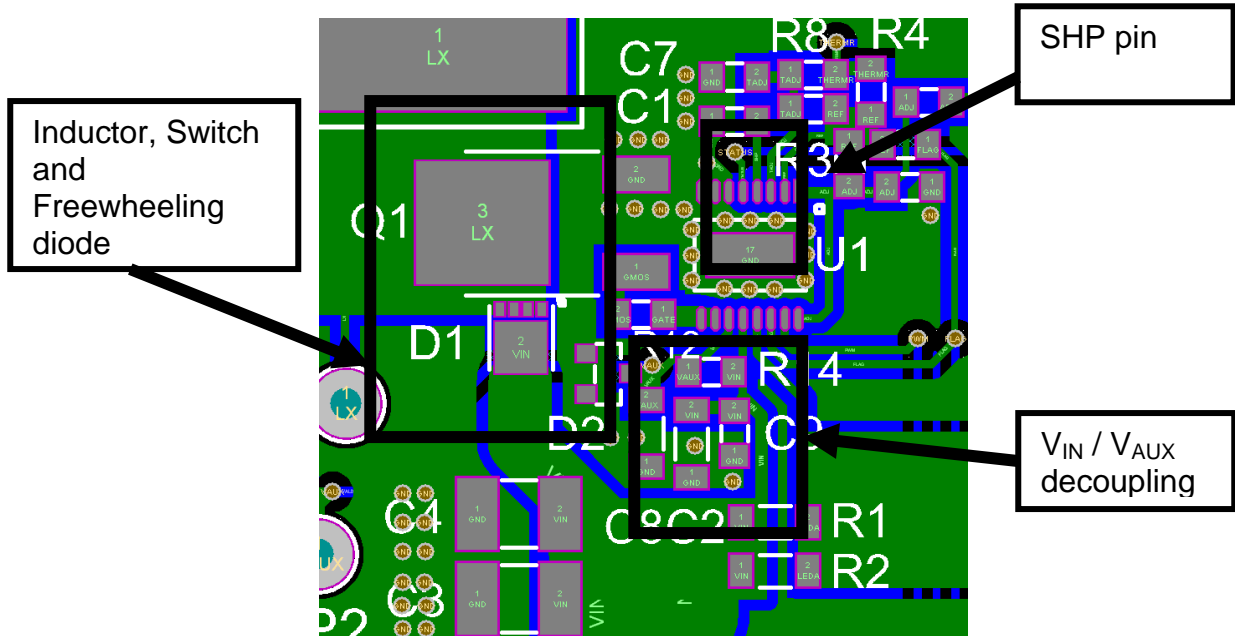
Figure 20. Circuit Layout
